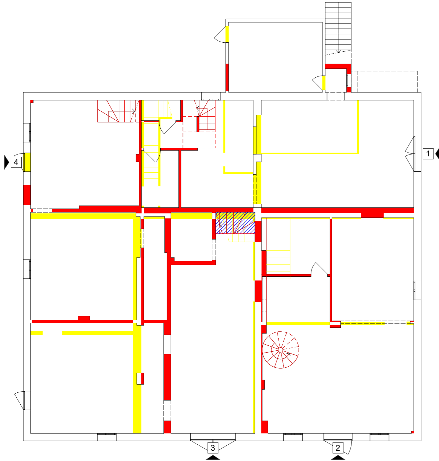
PIANO TERRA
